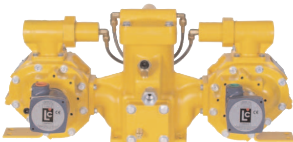
MA-4 LPG dispenser meter, dual
