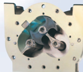
LC's three-rotor positive displacement measuring chamber.
